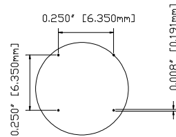
DETAIL A - DOT SPEC SCALE 5:1
