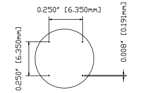
DETAIL A - DOT SPEC SCALE 5:1
